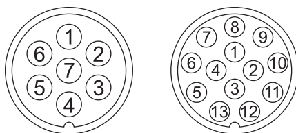
Fig. 1: Plug versions
